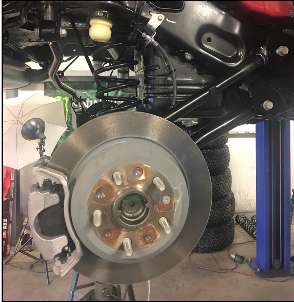
Rear Uppers and Rear Loweres Installed in the Vehicle
