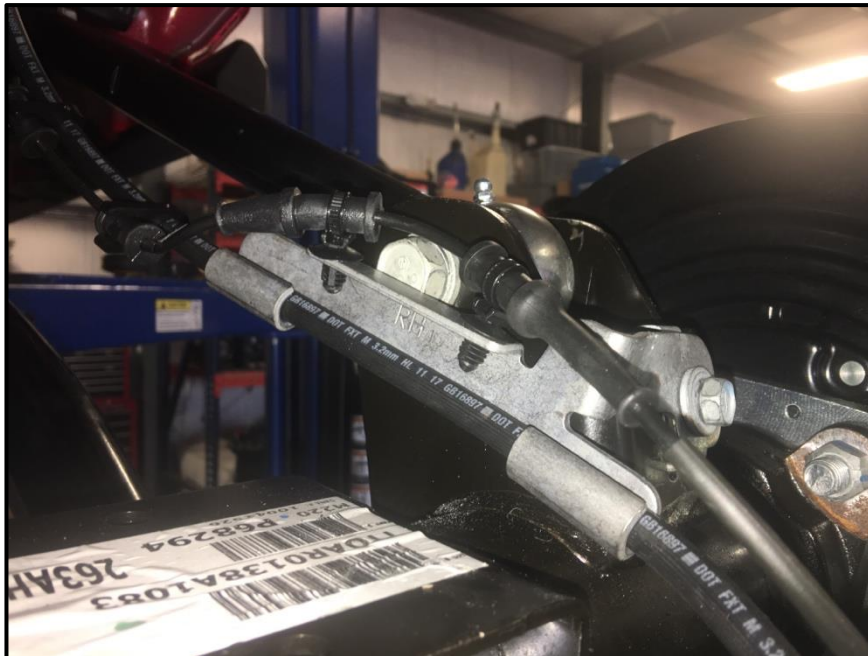
New Orientation for Rear Brake Line Brackets
