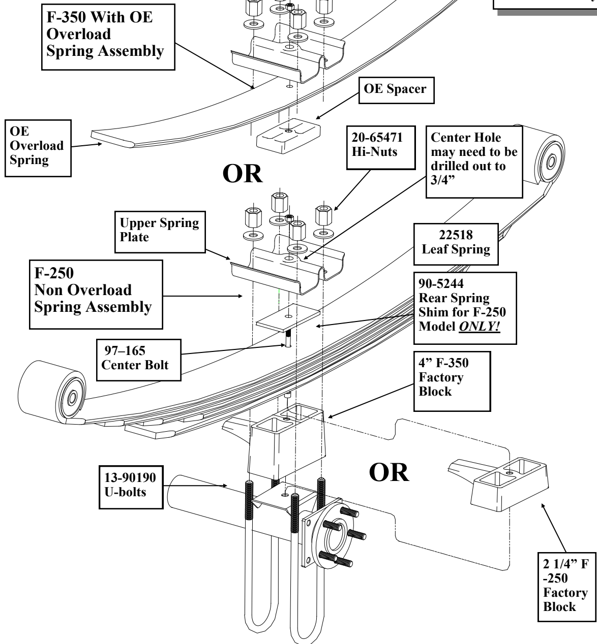
Illustration 10 Pro Comp Rear Spring Assembly
